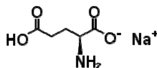
Fig. 1: Chemical formula of MSG
